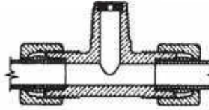
7C ANTI-FREEZE RESTRICTION TEE
